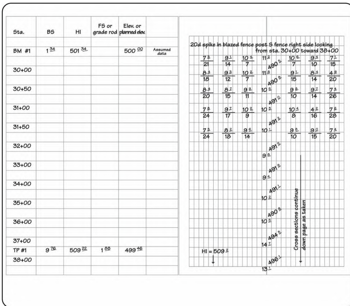
Figure 1-68: Survey Notes—Profile and Cross Section - continued
