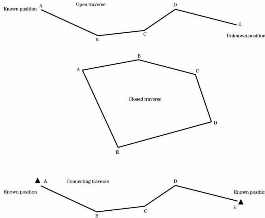
Figure 1-12: Open Traverse
