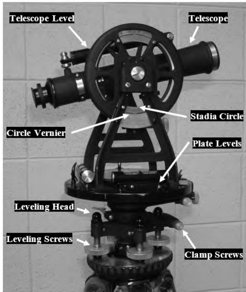
Figure 1-46: Engineer's Transit
